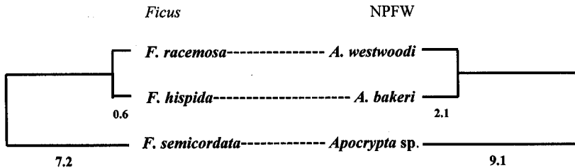
Fig. 1. The cluster analysis tree comparison between Ficus species and Apocrypta species (linkage distances are marked under branches).
