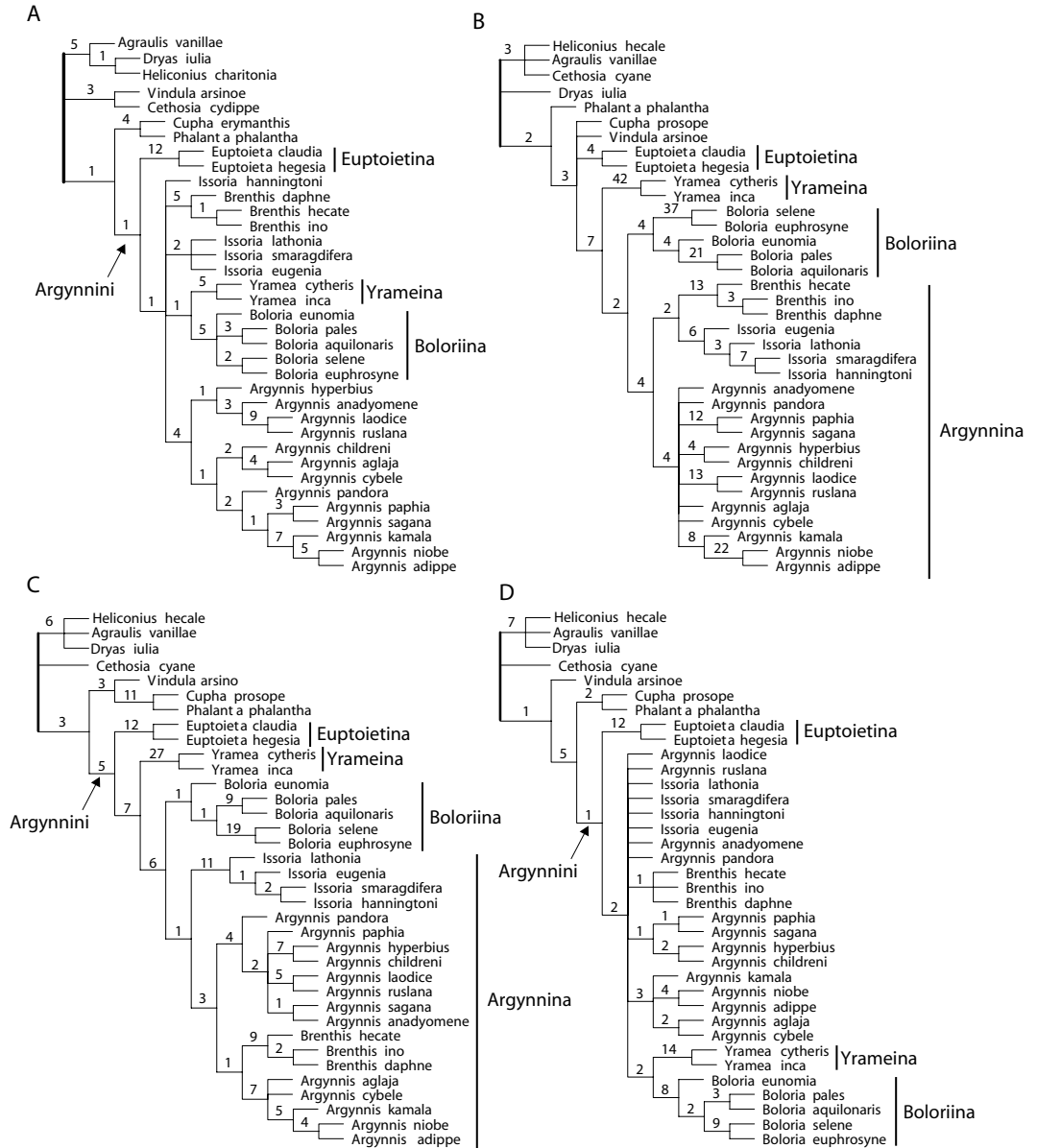
Fig. 1. Strict consensus trees from the separate analyses of the four datasets. A Morphology (8 trees, each 376 steps with CI = 0.41 and RI = 0.69), B COI (26 trees, each 2127 steps, CI = 0.36, RI = 0.43), C EF-1 \alpha (4 trees, each 772 steps, CI = 0.52, RI = 0.68), D wingless (6 trees, each 388 steps, CI = 0.51, RI = 0.63). The numbers above the nodes are Bremer support values.
